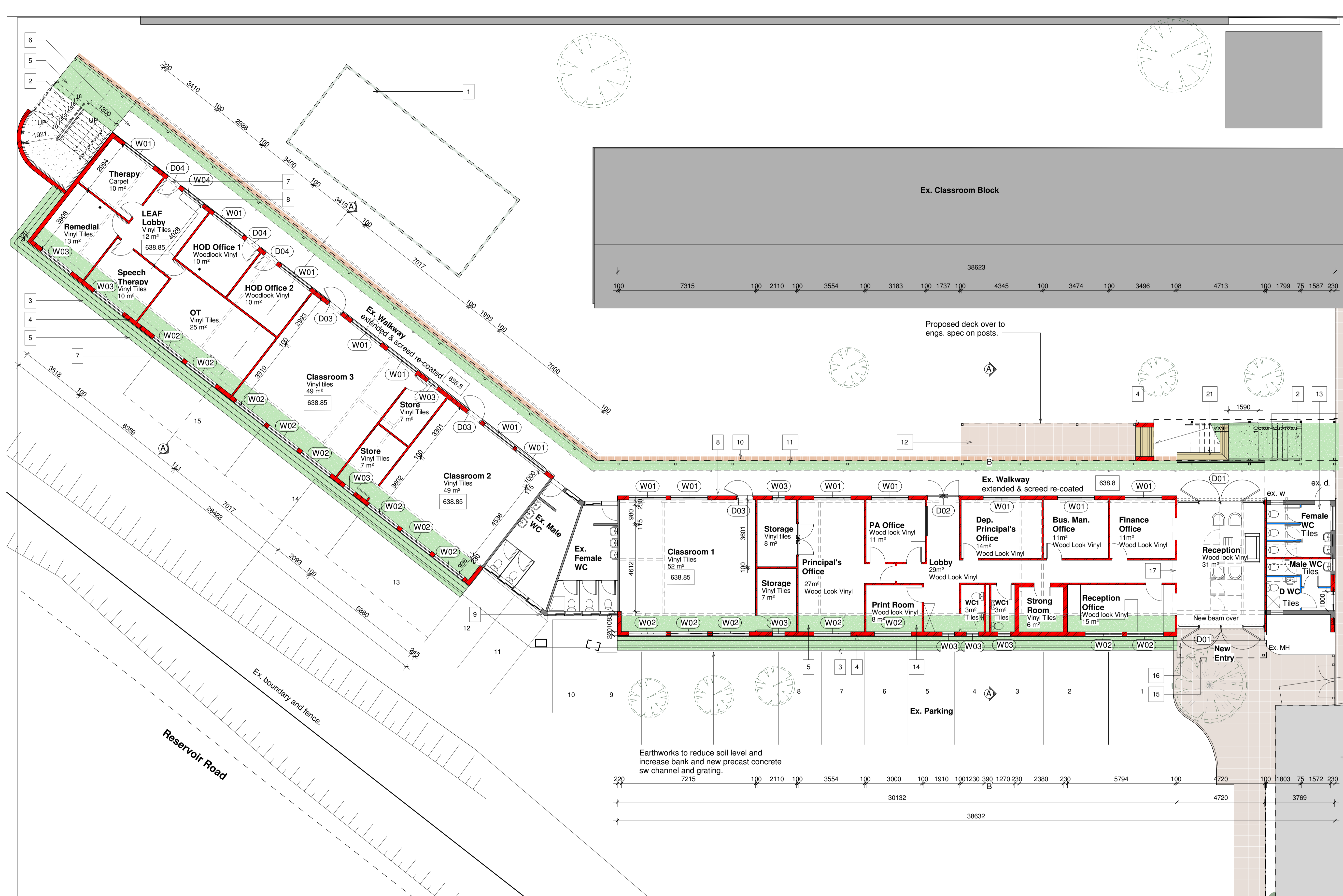
Grade 1 Block - Ground Floor Plan Scale 1 : 100
